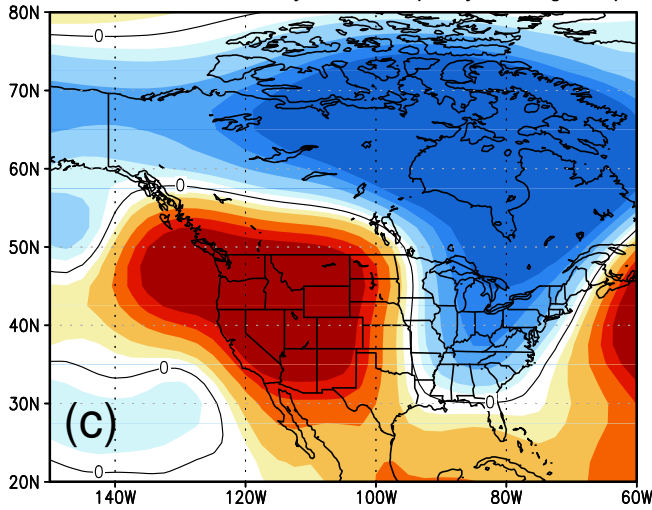
Composite GZ1000–500 Anomaly Zindex PC1 Dry–Wet (May–August)
