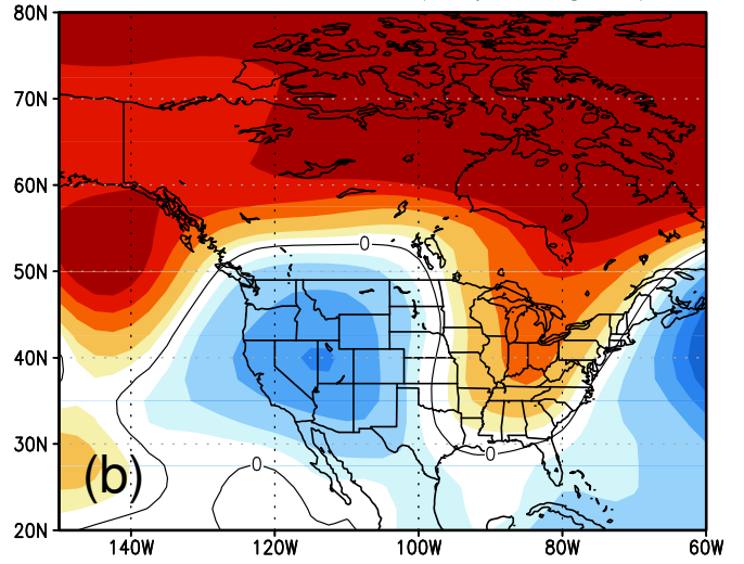
Composite GZ1000–500 Anomaly Zindex PC1 Wet (May–August)
