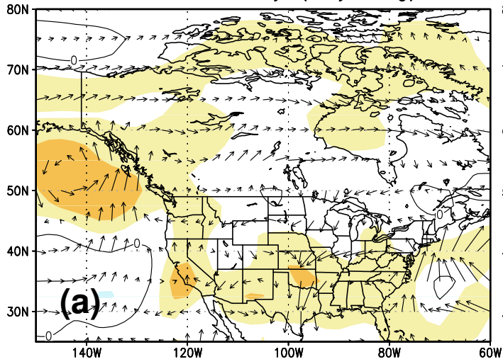
Composite Flux Anomaly 850 hPa Zindex PC1 Dry (May–Aug)
