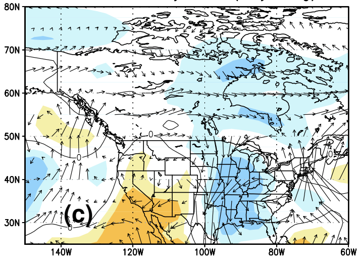
Composite Flux Anomaly 850 hPa Zindex PC1 Dry–Wet (May–Aug)
