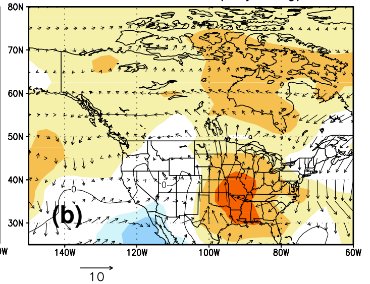
Composite Flux Anomaly 850 hPa Zindex PC1 Wet (May–Aug)
