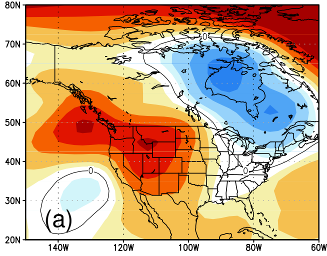
Composite GZ1000–500 Anomaly Zindex PC1 Dry (May–August)
